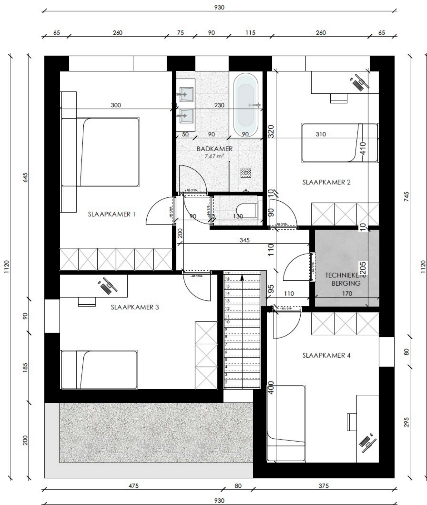
VERDIEPINGSPLAN LOT 1
